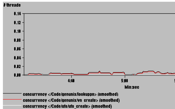
Figure 16: vn_create performance with both optimizations. The lookupn component has been reduced via a larger DNLC; the ufs_create component has been reduced because the open system call no longer uses the O_TRUNC flag. Note that ufs_create time is essentially zero.
