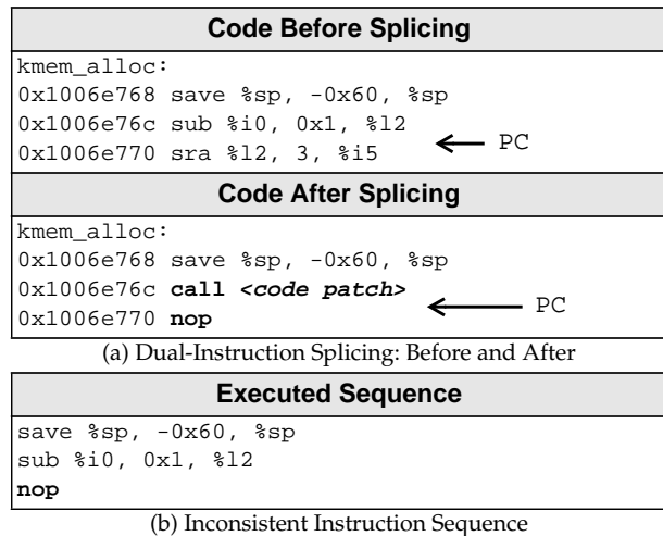
Figure 7: Why Multiple-Instruction Splicing is Hazardous return to, one of the instructions being replaced. If a hazard is detected, then splicing is deferred. This strategy is currently used by the Paradyn instrumentation system for user programs [9, 10]. However, it does not work in a kernel, for several reasons. First, pausing the kernel it is not allowed; even if it were, this would involve freezing all of the kernel threads (except, presumably, for the kerninstd thread, which is performing the splice), possibly disrupting critical background activities. Second, performing the necessary backtrace on all threads (of which there are thousands in the Solaris kernel) would be expensive. Third, even if pausing were possible and practical, a jump with an unanalyzable destination (such as a longjmp ) may jump to the middle of a splice sequence, resulting in the execution of an inconsistent code sequence. A fourth problem with multiple-instruction splicing occurs when the instrumentation point is at the end of a basic block B_1 . Some of the splice sequence spills over into the next basic block B_2 . If B_2 is reachable from another block (say, by a branch from block B_3 ), then code taking the path ( B_3 , B_2 ) will execute the second half of a splice sequence, an inconsistent code sequence which can crash the kernel. For these reasons, we conclude that fine-grained dynamic instrumentation is unsafe when using multiple-instruction splicing.
