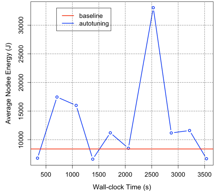
Autotuning SW4lite on 1024 Nodes on Theta
