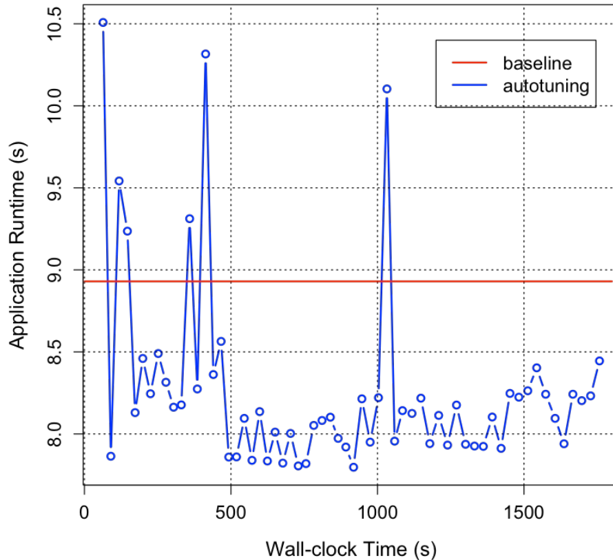
Autotuning SWFFT on 4096 Nodes on Summit
