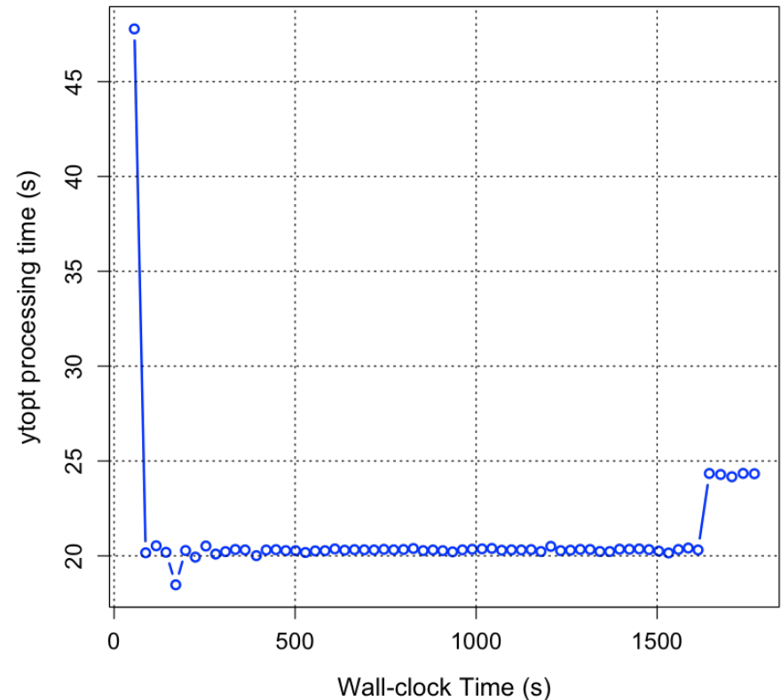
Autotuning AMG on 4096 Nodes on Summit
