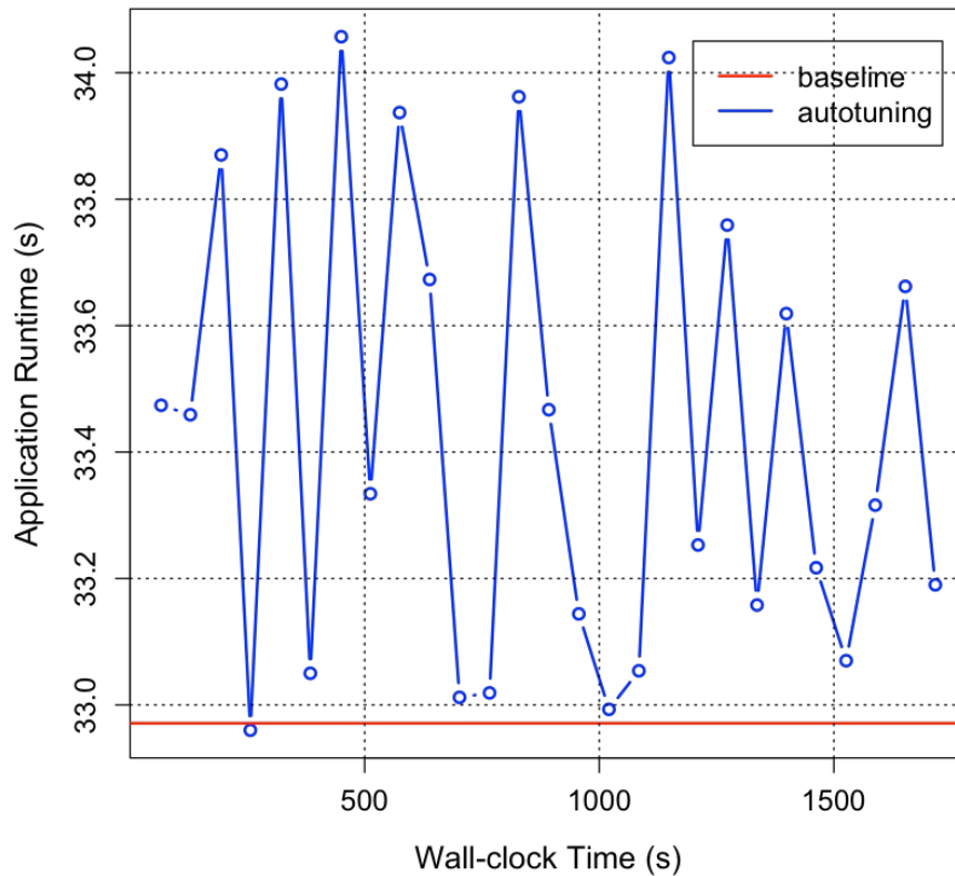
Autotuning SWFFT on 4096 Nodes on Theta
