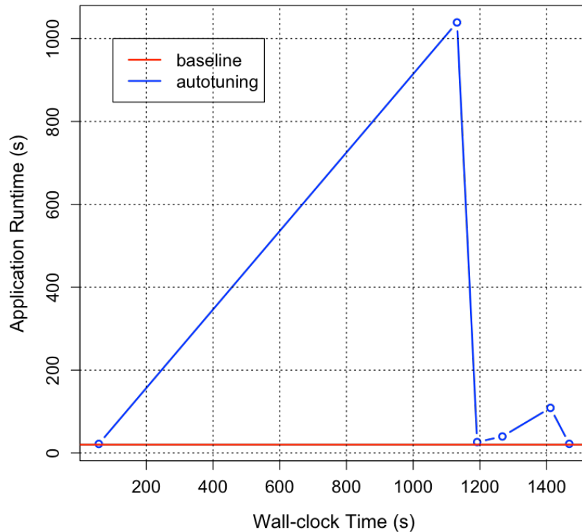
Autotuning AMG on 4096 Nodes on Theta
