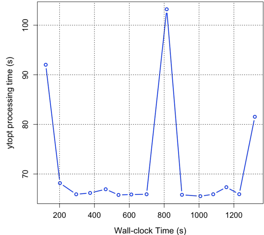
Autotuning SW4lite on 1024 Nodes on Summit
