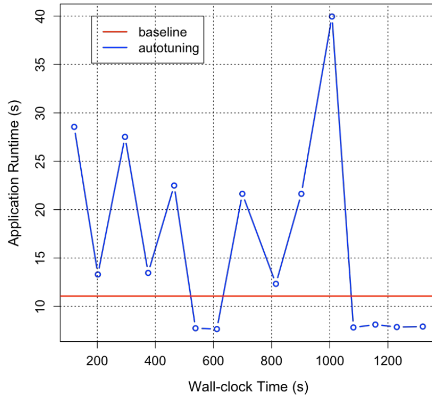
Autotuning SW4lite on 1024 Nodes on Summit
