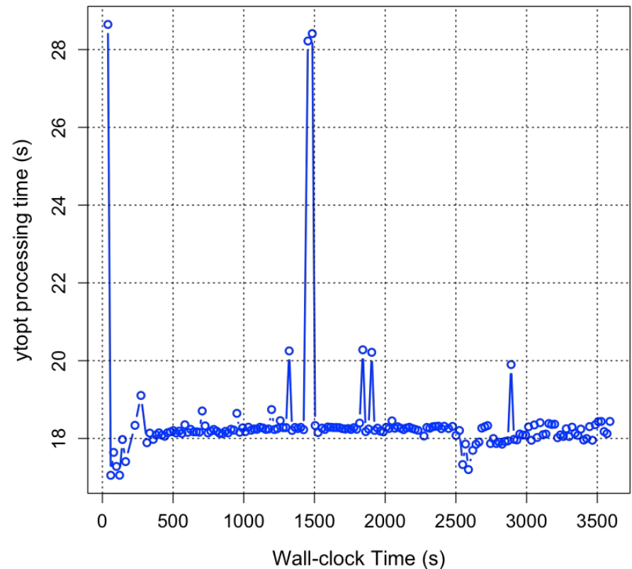
Autotuning OpenMP Offload XSBench on a Summit Node
