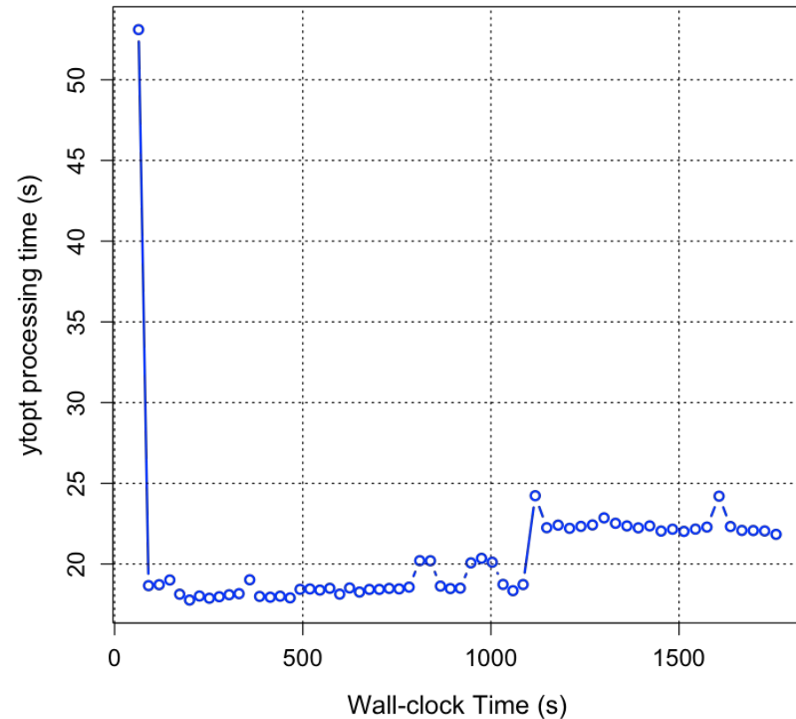
Autotuning SWFFT on 4096 Nodes on Summit
