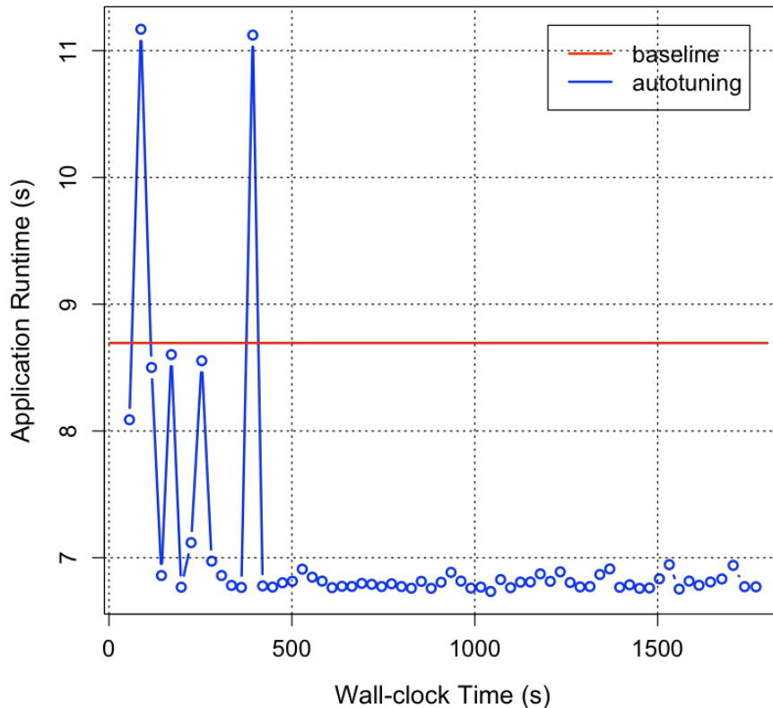
Autotuning AMG on 4096 Nodes on Summit
