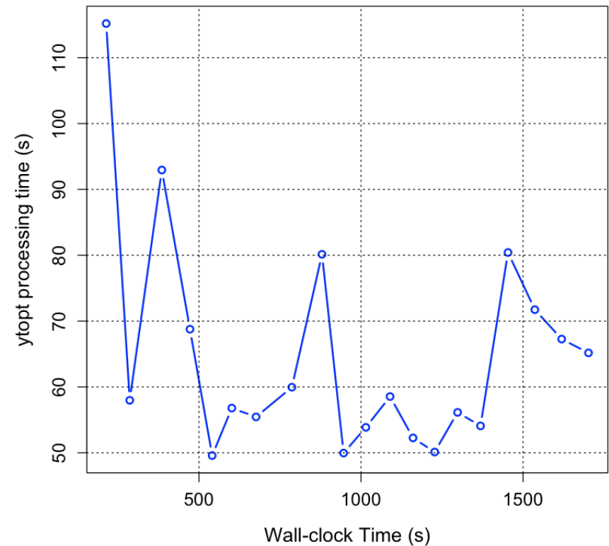
Autotuning XSBench on 4096 Nodes on Summit
