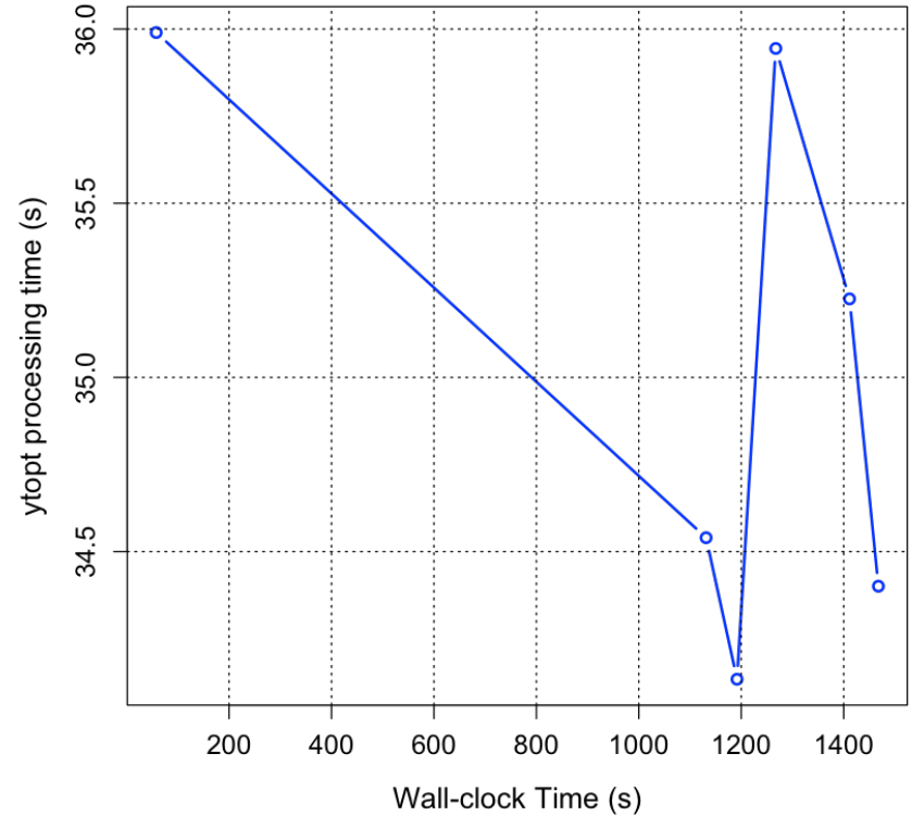
Autotuning AMG on 4096 Nodes on Theta
