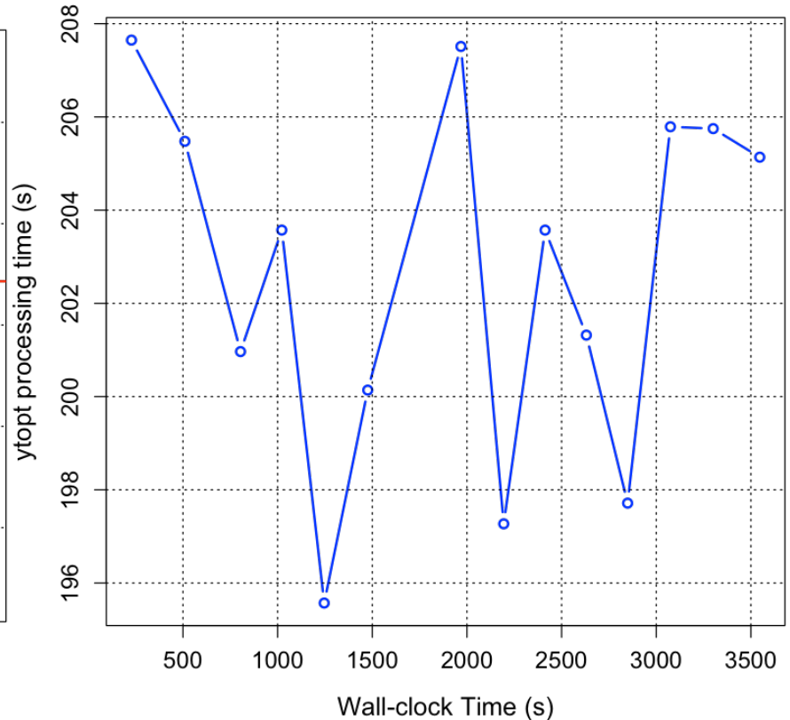
Autotuning SW4lite on 1024 Nodes on Theta
