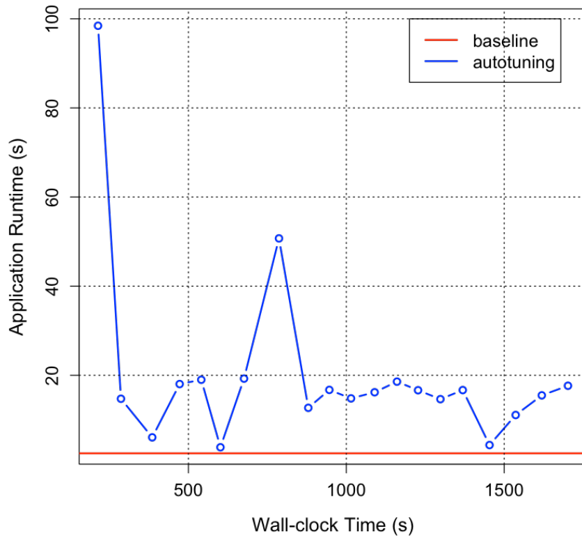
Autotuning XSBench on 4096 Nodes on Summit
